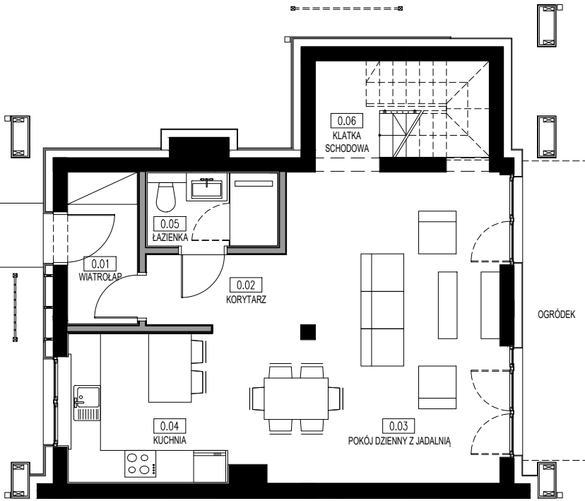
PARTER
